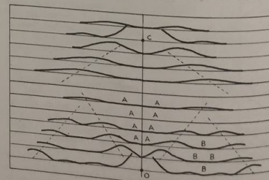
Fig. 2. Diffraction pattern of system of helices corresponding to structure of deoxypentose nucleic acid. The squares of Bessel functions are plotted about O on the equator and on the first, second, third and fifth layer lines for half of the nucleotide mass at a given radius being proportional to the radius, the C on the tenth layer line similar functions are plotted for an outer diameter.
